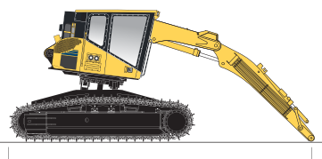
4 Bar Arm, Std Boom = 25'2" (7671 mm)
